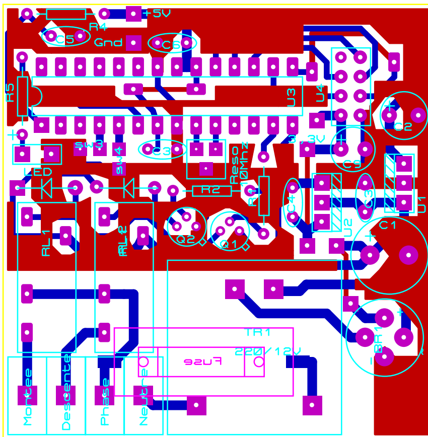
Version 8 - ATmega328P
