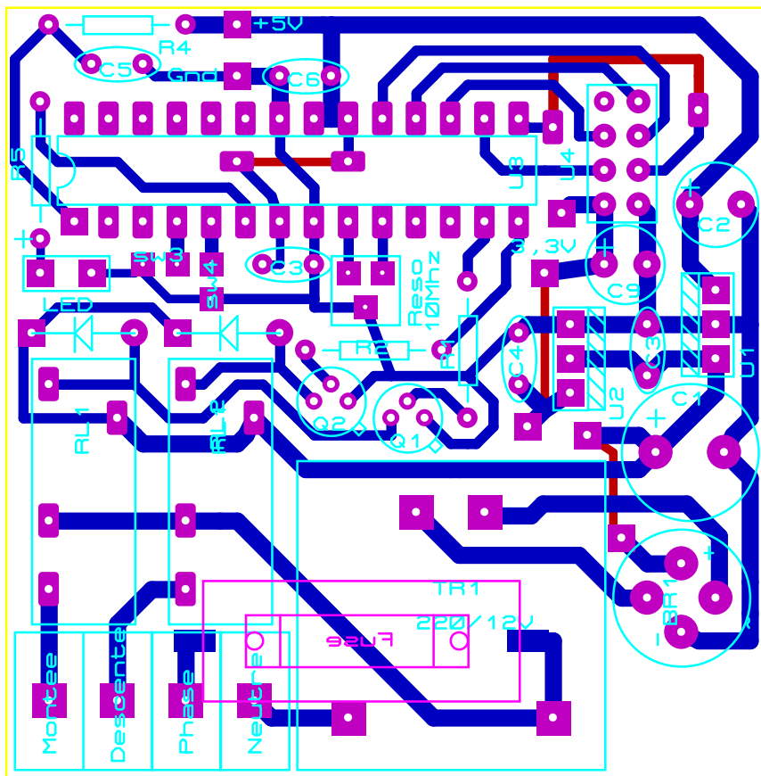
Version 7 - ATmega328P
